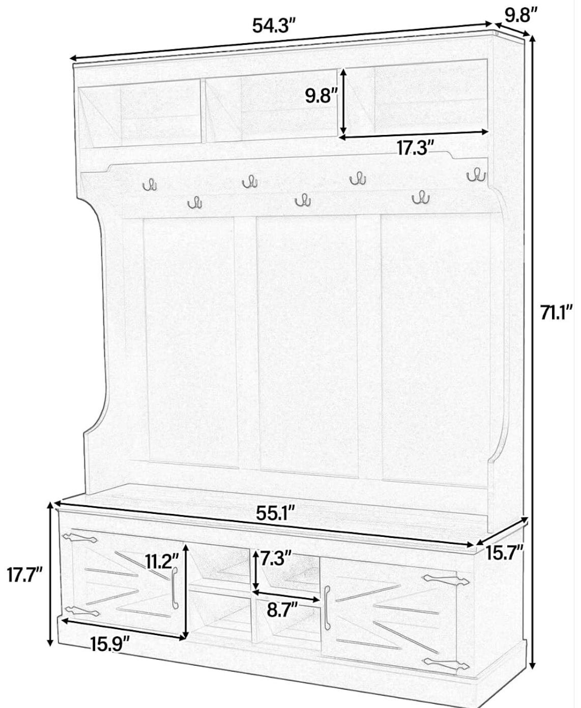
Figure 5: Product Dimensions. This diagram provides a detailed view of the hall tree's measurements in inches, including overall height, width, depth, and internal compartment sizes.
