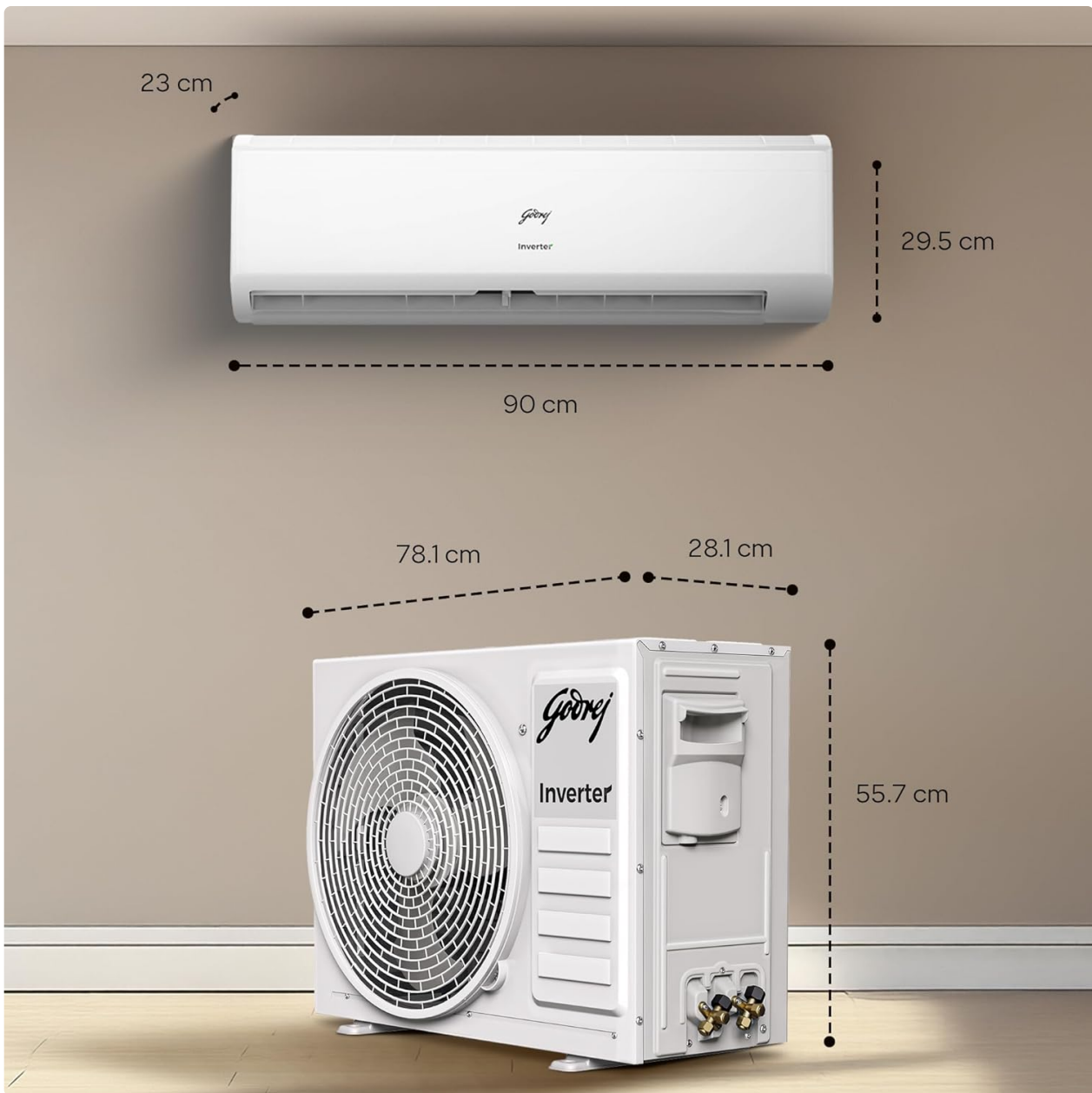
Image: Diagram showing the dimensions of both the indoor and outdoor units of the Godrej Inverter Split AC.
