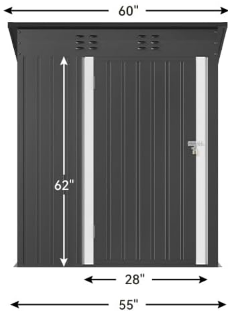
Image: Detailed dimensions of the COMHOMA 5'x3' storage shed.
