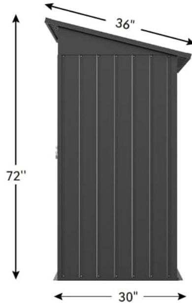
Image: Detailed dimensions of the COMHOMA 5'x3' storage shed.
