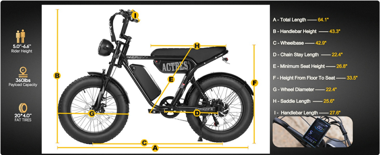
Image: Detailed dimensions of the electric bike for reference.
