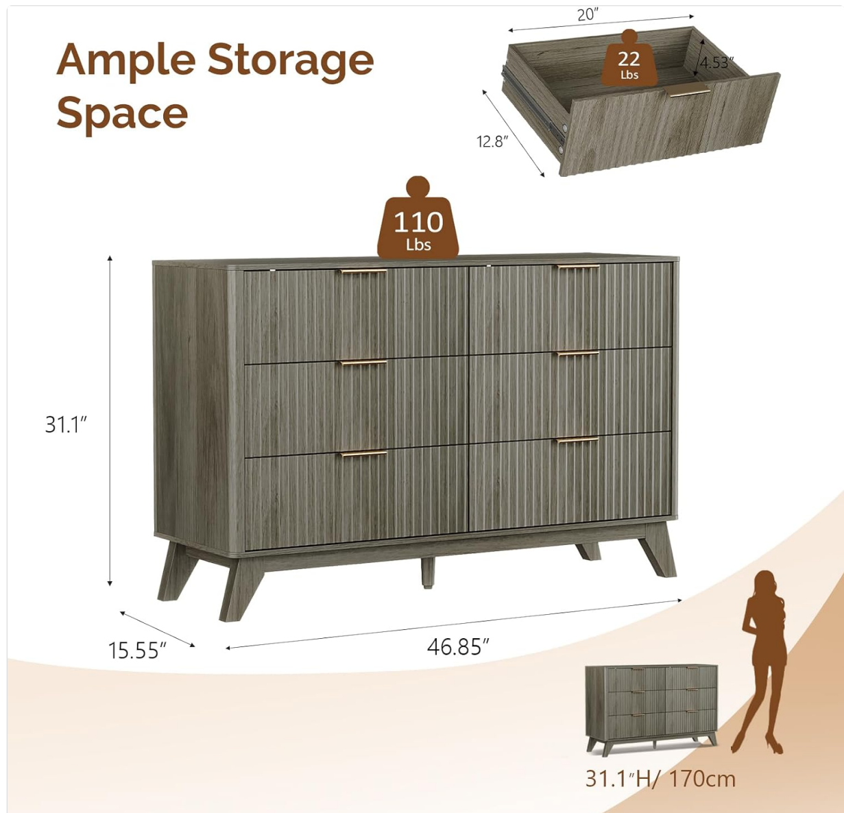
Image 3.1: Dresser dimensions and weight capacities. This image illustrates the overall dimensions of the dresser (46.85"W x 15.55"D x 31.1"H), the drawer depth (12.8"), and the weight limits for the tabletop (110 lbs) and each drawer (22 lbs).
