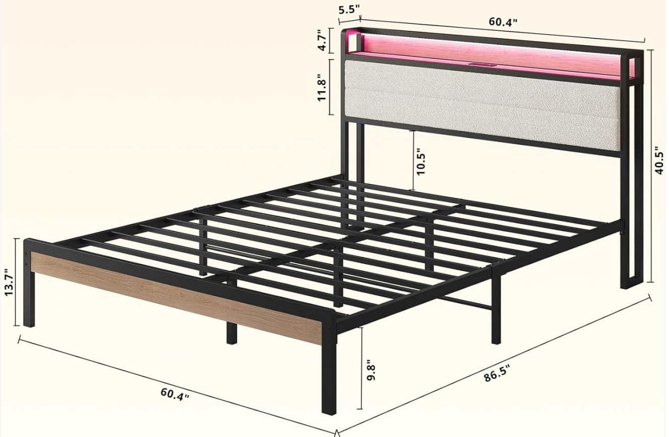
Image: Dimensional drawing of the LIKIMIO Queen Bed Frame, indicating overall length, width, and height, as well as specific measurements for the headboard and under-bed clearance.
