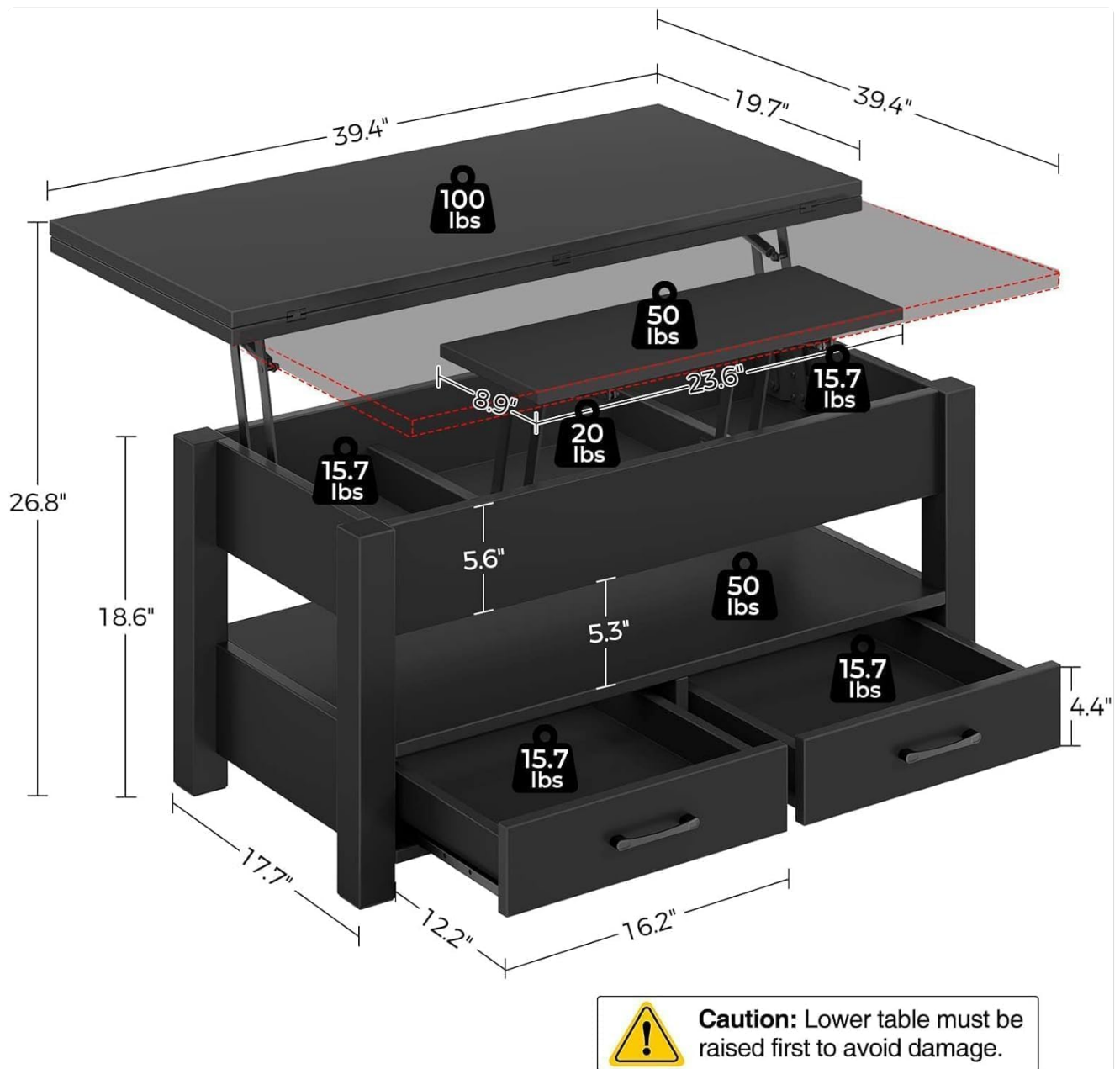
Figure 1: Product Dimensions and Weight Capacities. This diagram illustrates the overall dimensions of the coffee table and the maximum weight load for each section, including the lift tops, hidden compartments, open shelf, and drawers.
