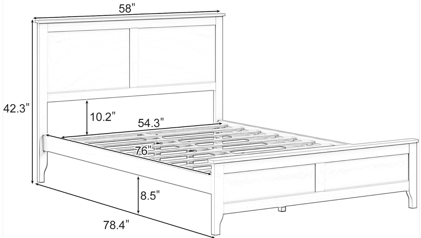
Figure 2.1: Components of the bed frame before assembly.
