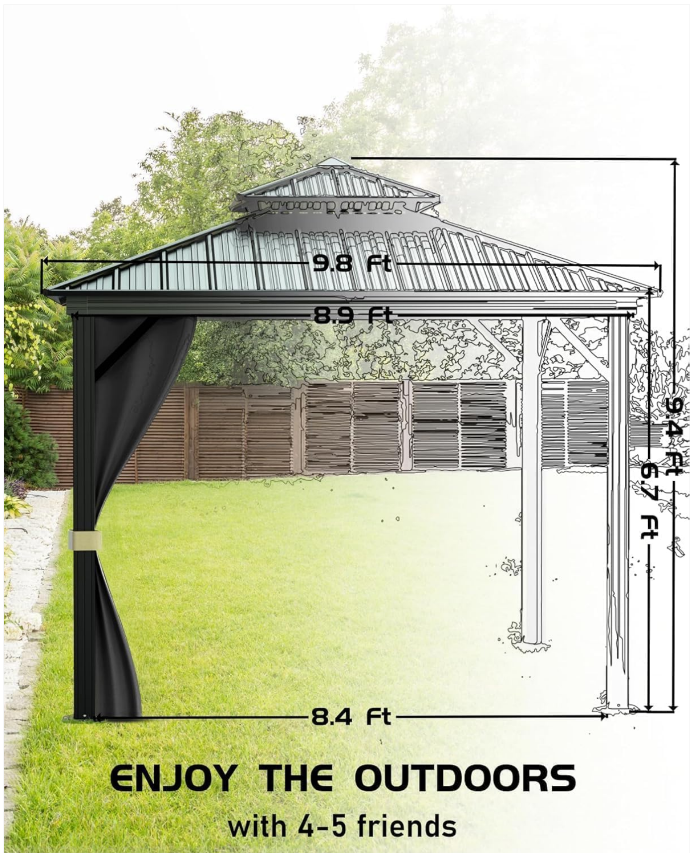
Figure 4.1: Gazebo dimensions for planning your setup location.
