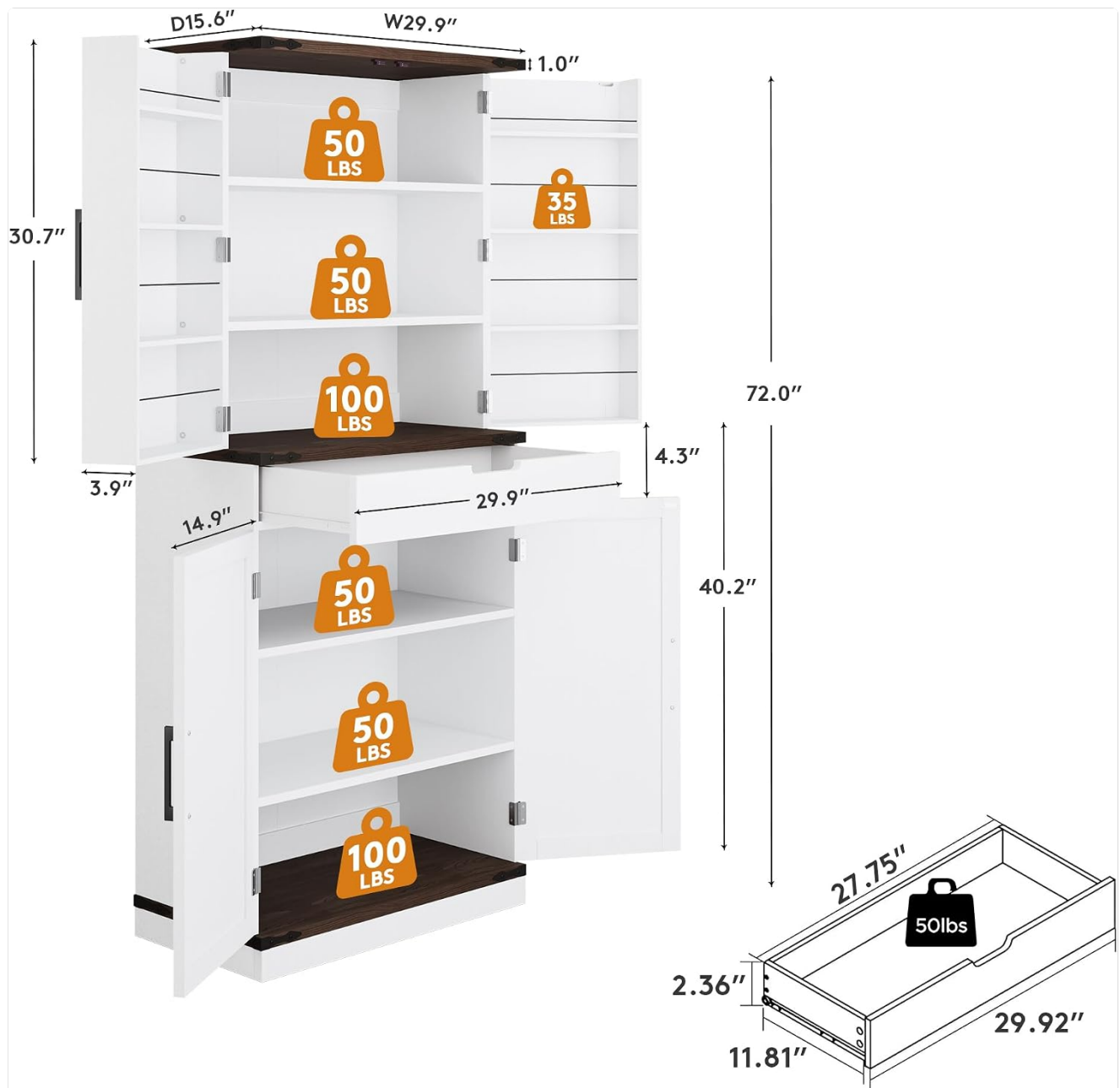
Image 4.1: Detailed dimensions and individual shelf/drawer weight capacities for planning and assembly.
