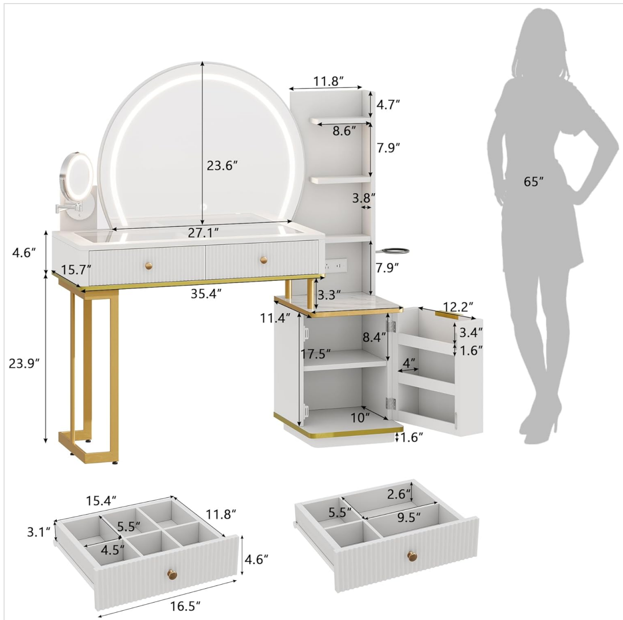
Image: Detailed diagram showing the dimensions of the vanity desk and its various components.
