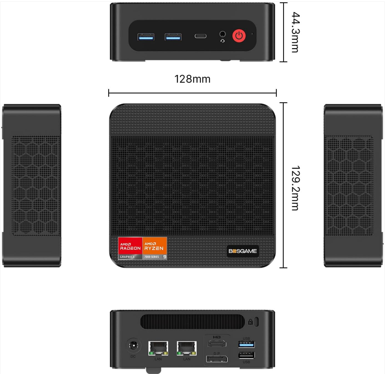
Image: Front and rear view of the BOSGAME P3 Pro Mini PC, illustrating port locations and overall dimensions.
