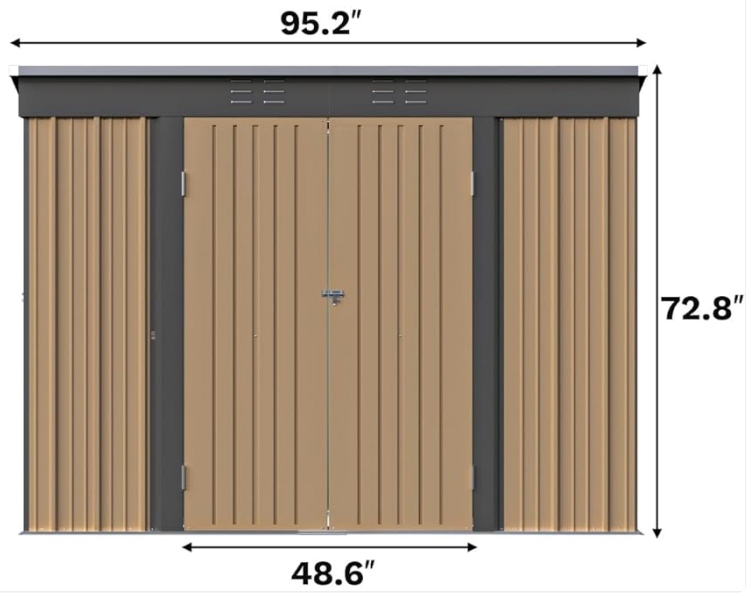
Image 4.1: Dimensional diagram of the Patiowell 8x4 FT storage shed, illustrating its length, width, and height.
