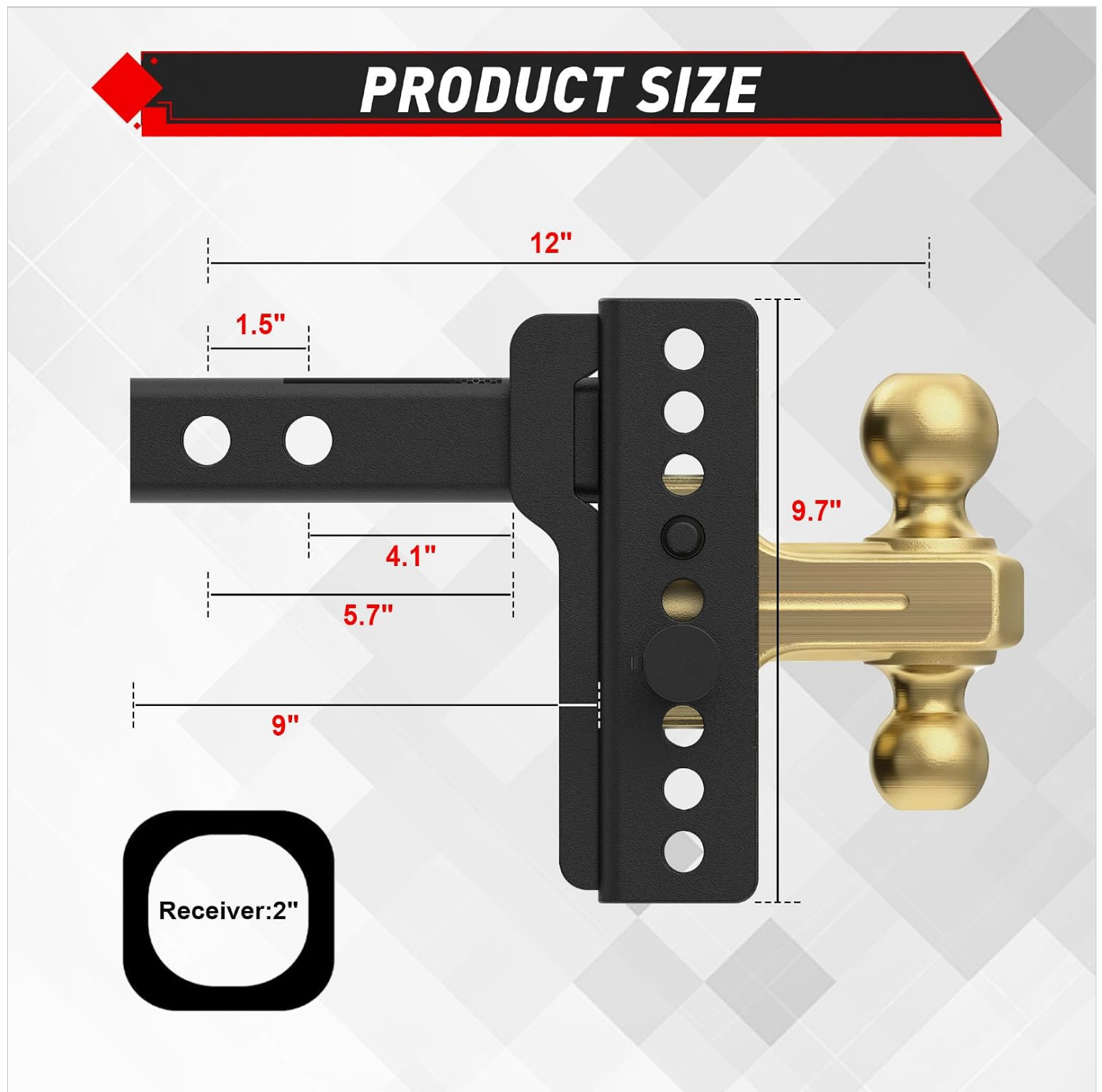
Figure 3.2: Detailed dimensions of the TYT Adjustable Truck Trailer Hitch, indicating overall length, receiver insertion depth, and height adjustments.
