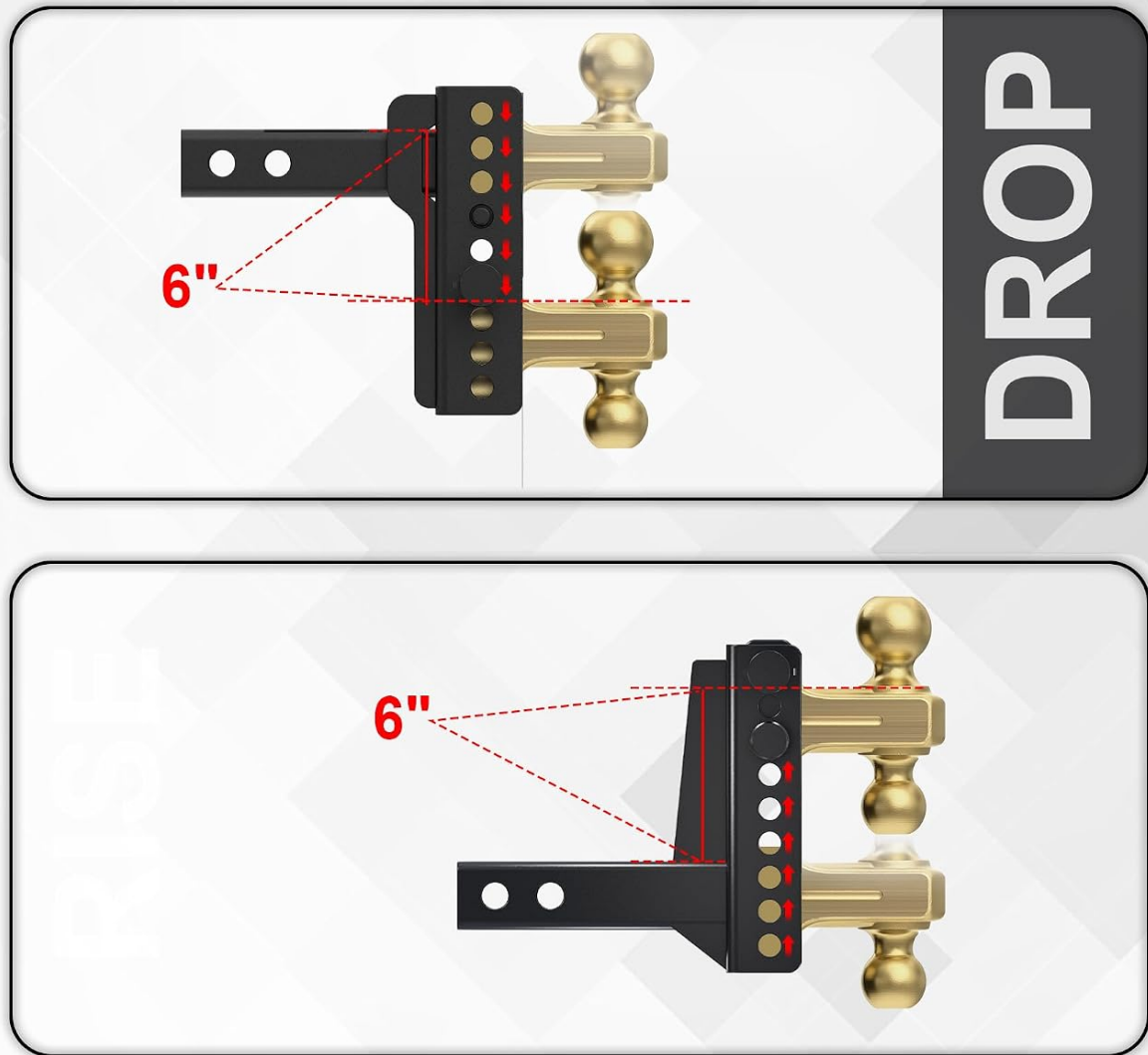
Figure 4.1: Illustration of the 6-inch drop and rise adjustment capability of the hitch, demonstrating how to position the ball mount for level towing.
