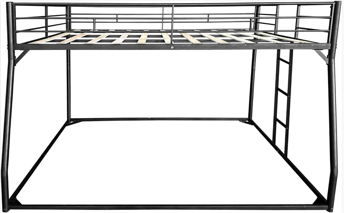
Image: Front view of the assembled bunk bed frame, illustrating the Full XL over Queen configuration.
