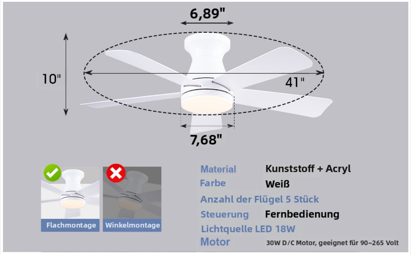
Image: Technical diagram illustrating the dimensions (41 inches diameter, 10 inches height) and key specifications of the Kviflon ceiling fan, including material (Plastic + Acrylic), color (White), 5 blades, remote control, 18W LED light source, and 30W D/C motor.
