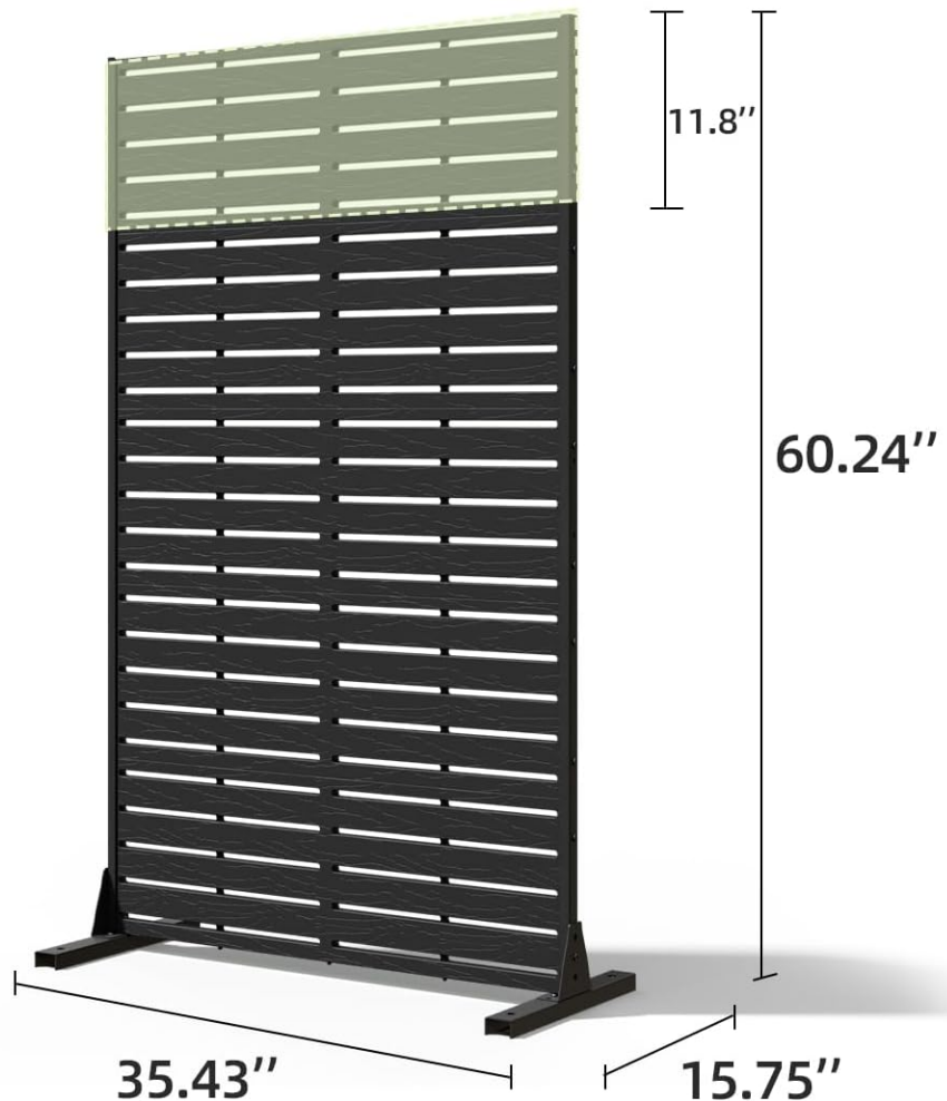
Figure 3: Product dimensions and scale reference.
