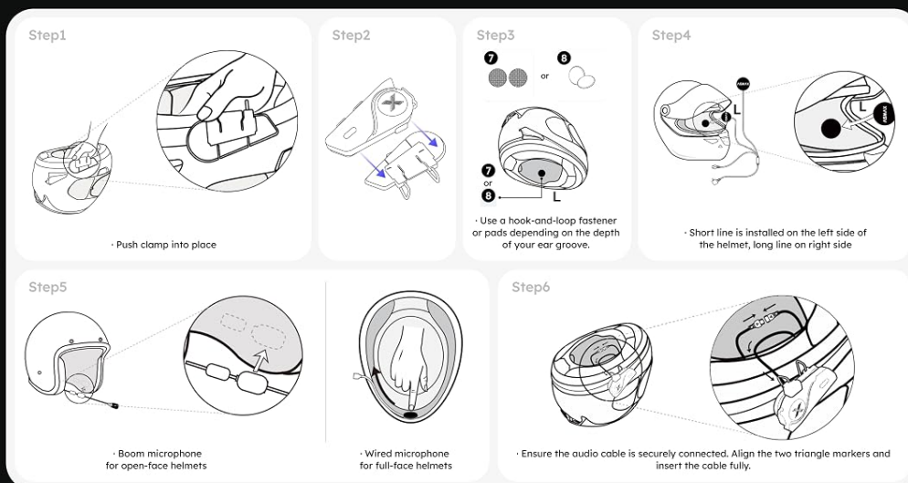
Figure 2: Installation Steps for MAXRUNON D9
