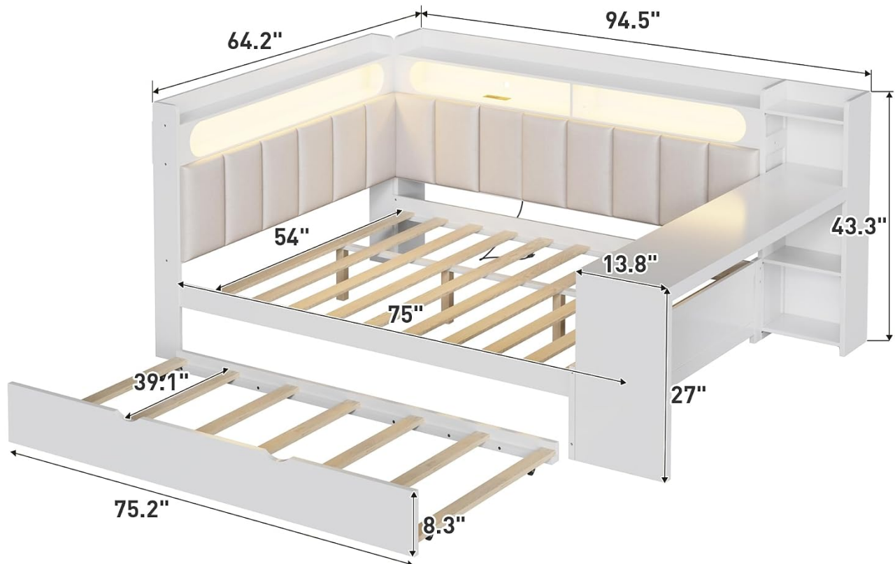
Image 3.1: Detailed dimensions of the SOFTSEA Full Size Corner Bed in inches.
