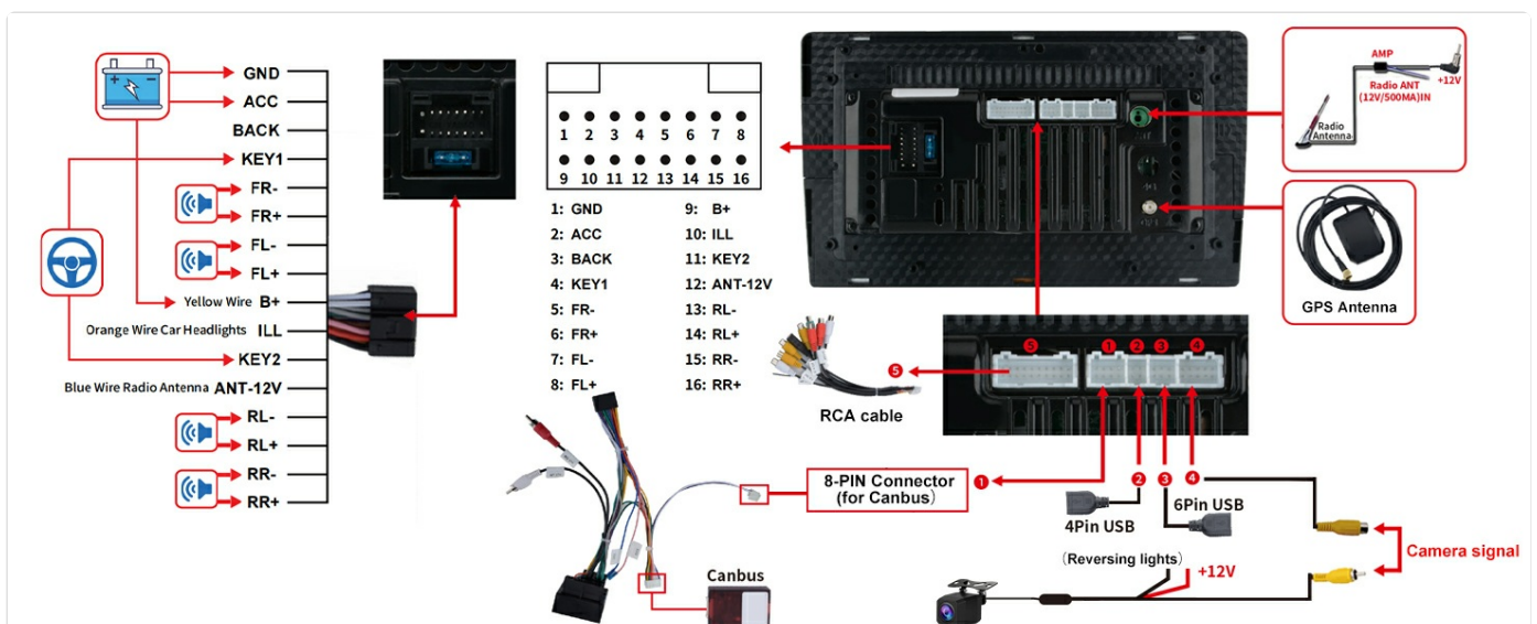
Figure 3.2: General Wiring Diagram. This diagram shows the connections for the main unit, power, speakers, and accessories.
