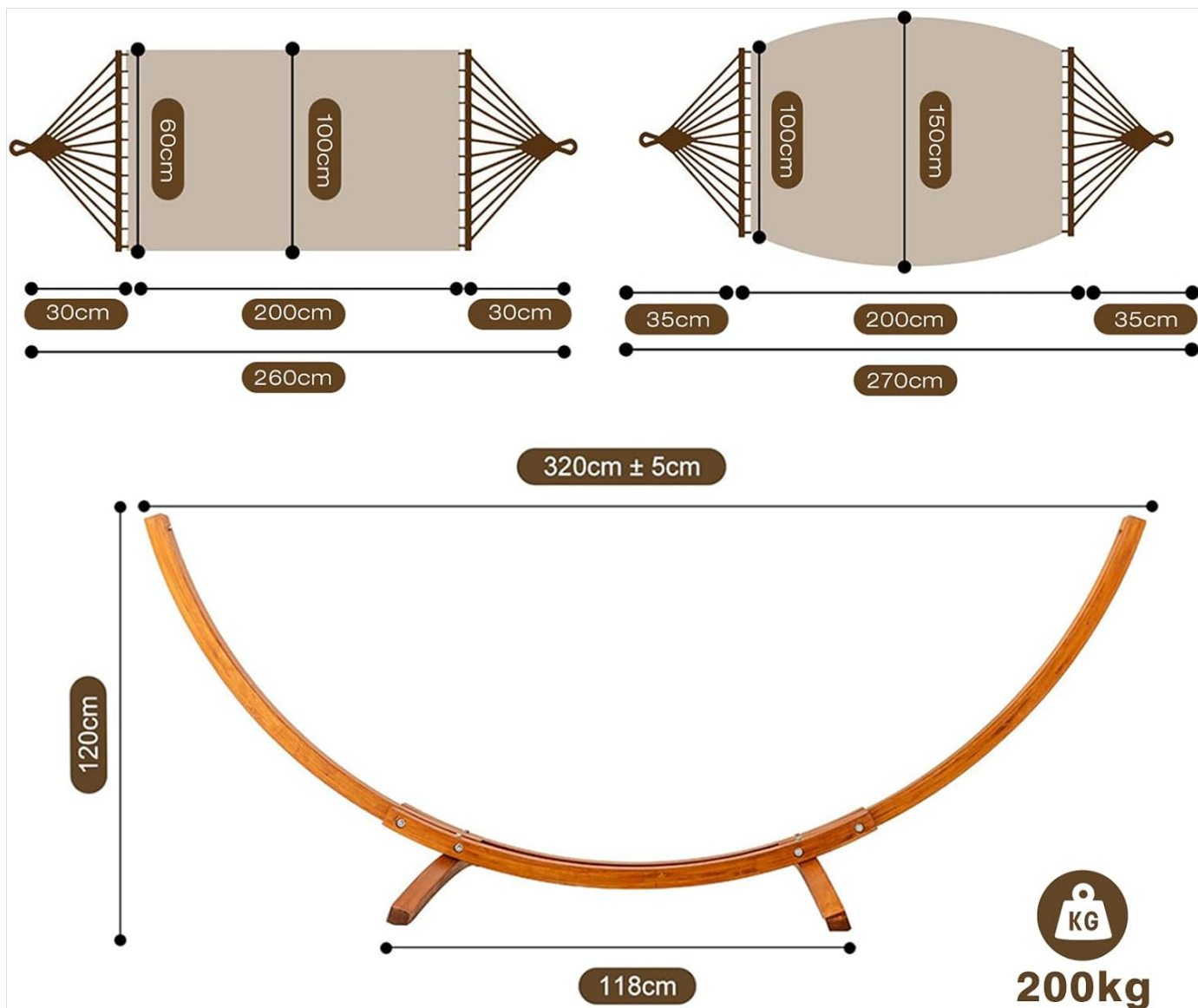
Image 8.1: Detailed dimensions of the hammock and stand.
