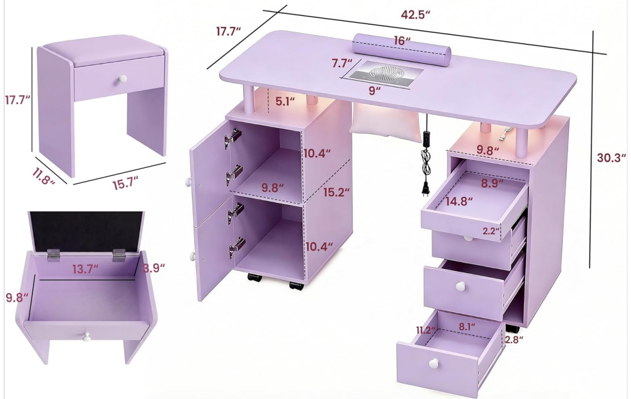
Figure 7: Detailed product dimensions.
