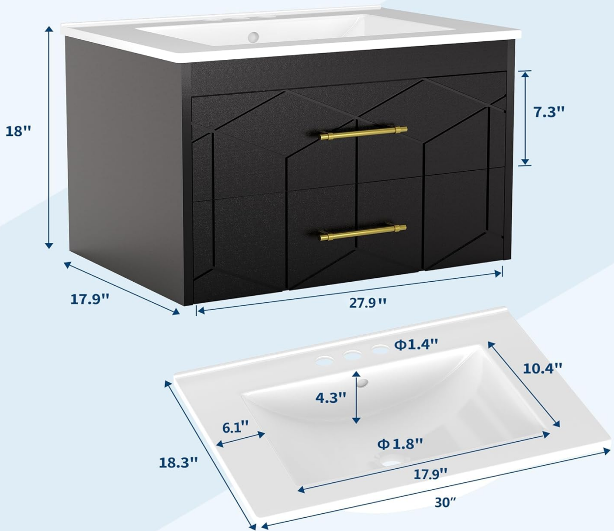
Figure 4.1: Product Dimensions. Refer to this diagram for precise measurements during installation.
