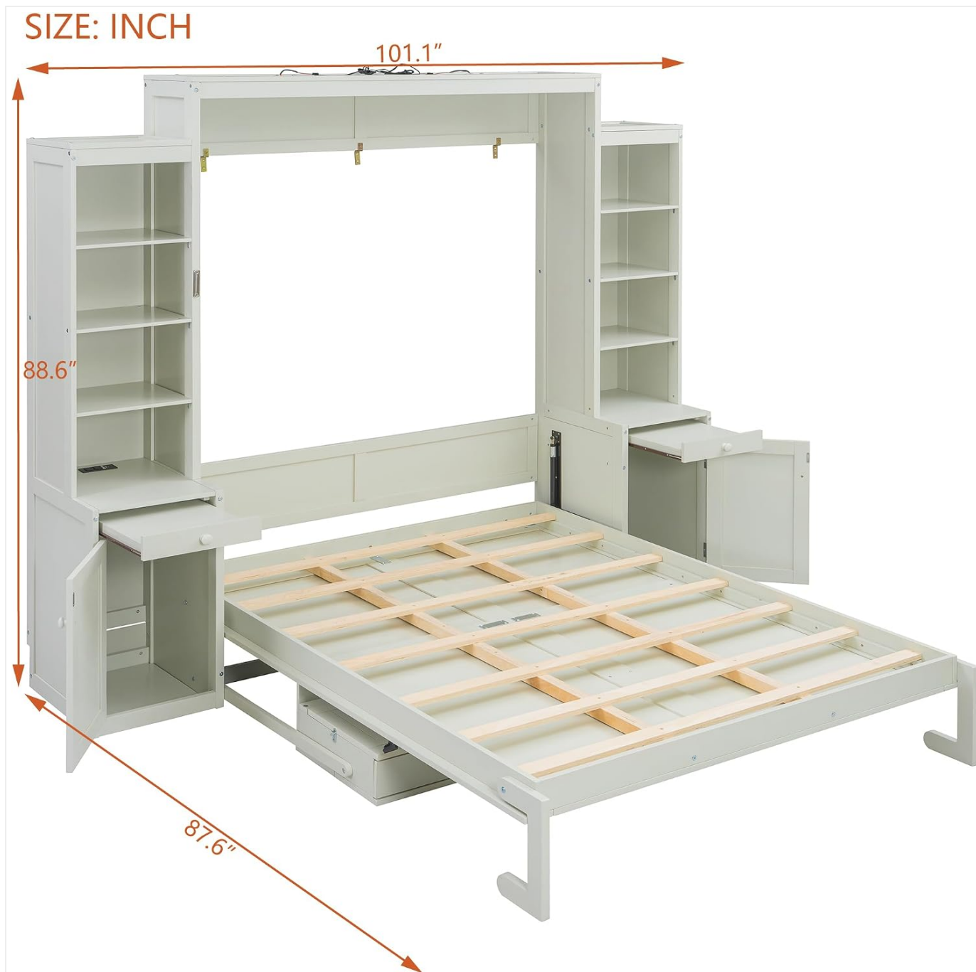
Image: A detailed diagram showing the overall dimensions of the Brabrety Queen Size Murphy Bed, including length, width, and height measurements in inches. This helps in planning placement and understanding the product's footprint.
