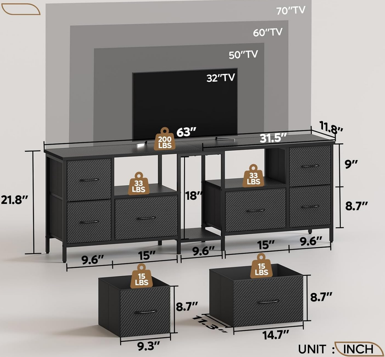
Image: Diagram illustrating the overall dimensions of the TV stand and the weight capacities for the tabletop, shelves, and drawers.
