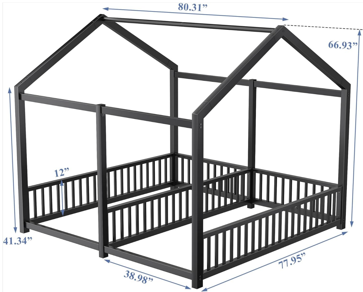
Image 1: Assembled bed frame with key dimensions indicated. The bed features a house-shaped roof and low guardrails.
