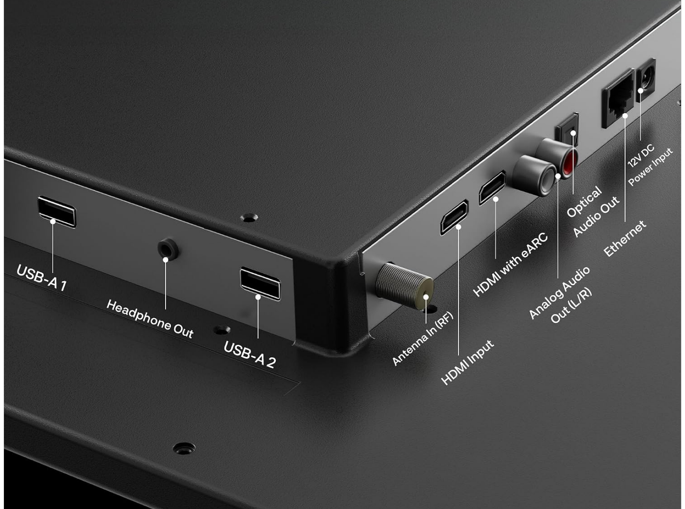
Image: Detailed diagram of the TV's connectivity ports, including USB-A 1, Headphone Out, USB-A 2, Antenna In (RF), HDMI Input, HDMI with eARC, Analog Audio Out (L/R), Optical Audio Out, Ethernet, and 12V DC Power Input.
