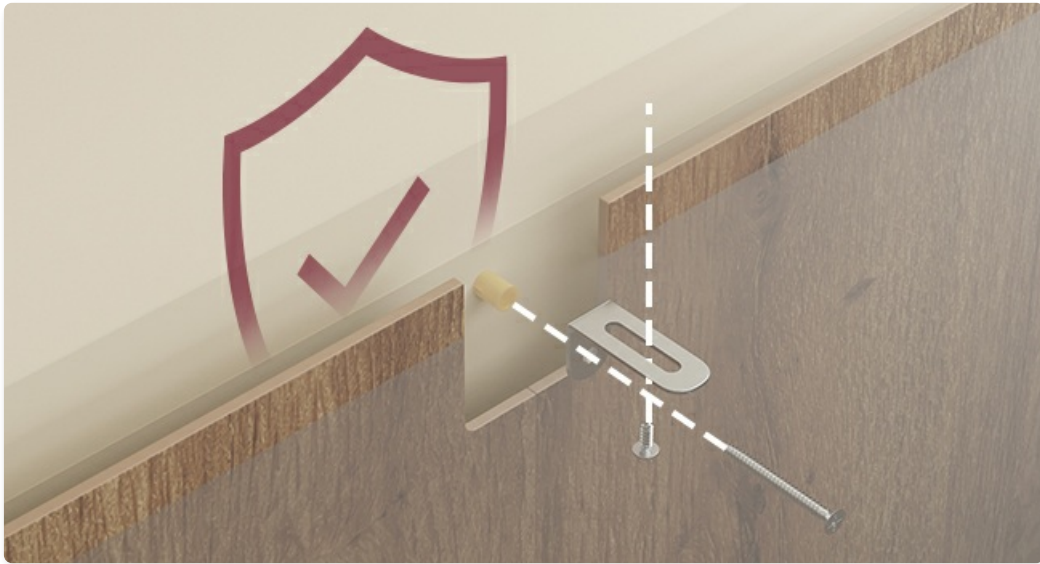
Illustration of the anti-tip kit installation, demonstrating how to securely fasten the cabinet to the wall.
