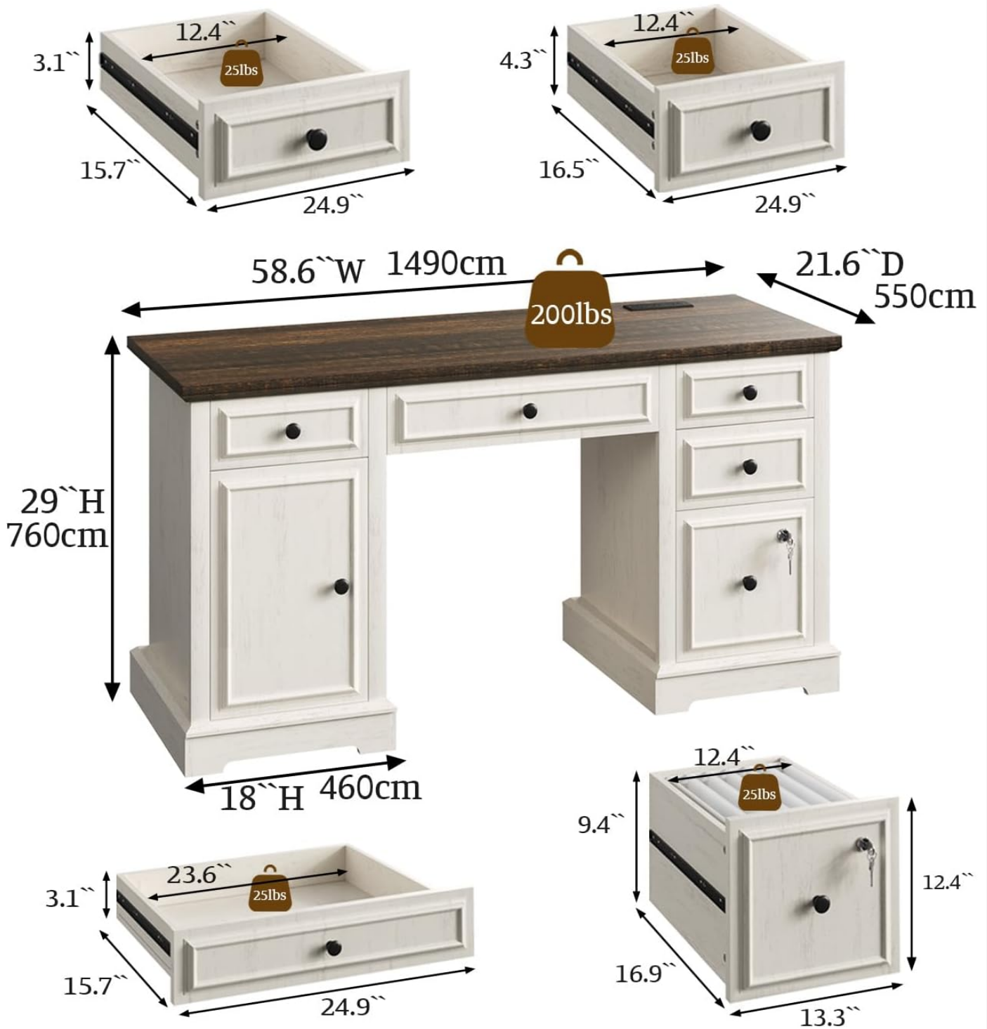
Image: Detailed diagram showing the dimensions of the desk and its various compartments.
