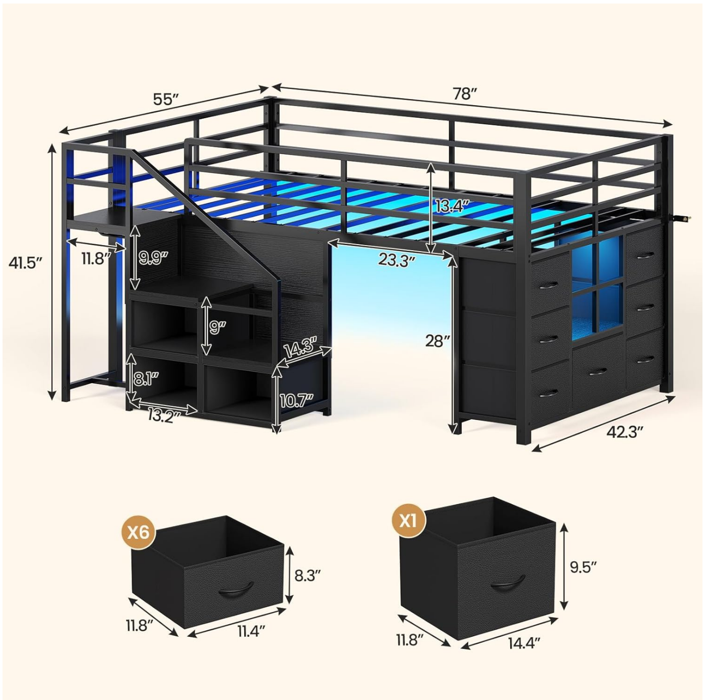
Figure 1: Overview of the BTHFST Low Loft Bed with key dimensions and storage components.
