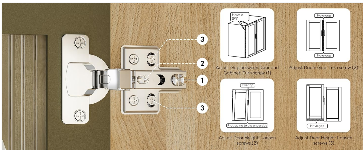
A diagram illustrating the soft-close hinges and how to adjust them for proper door alignment.
