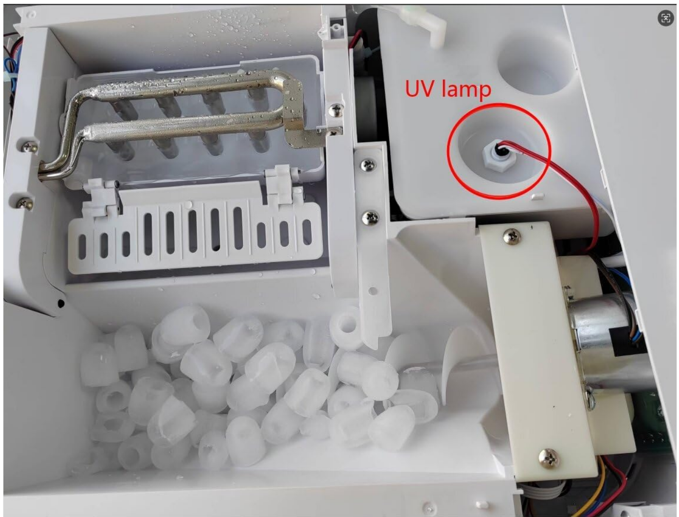
Image: Internal view of the ice maker, showing ice cubes and the UV lamp.
