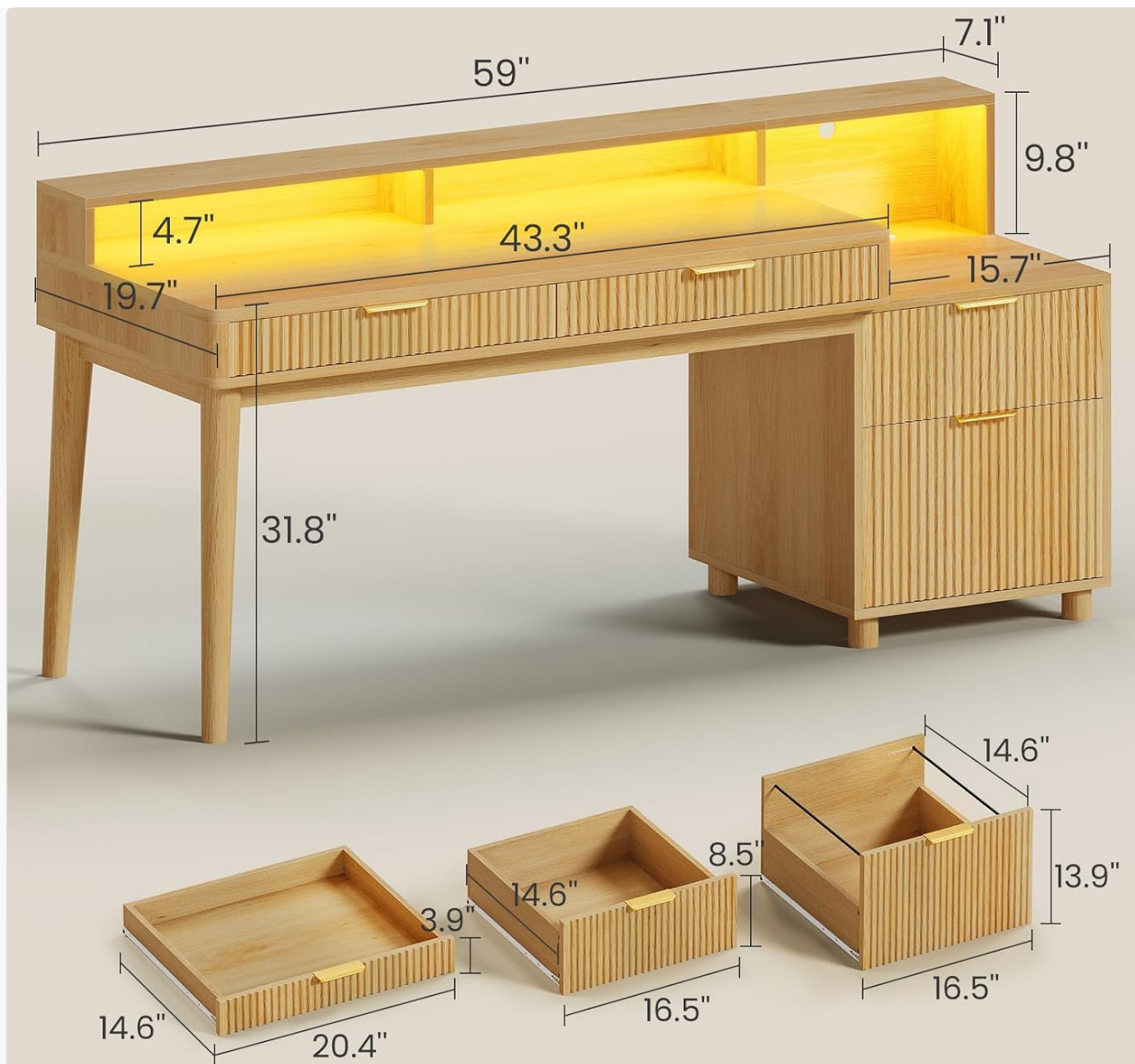
Image 8.1: Key dimensions of the computer desk.
