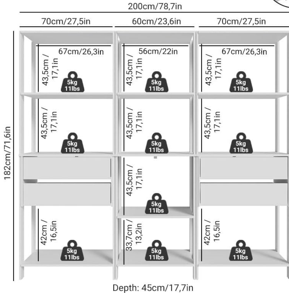
Diagram illustrating the overall and individual compartment dimensions of the pantry, including weight capacity per shelf and drawer (11 lbs / 5 kg).
