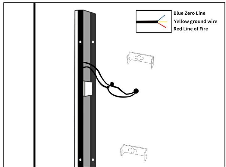
Image: Diagram showing the electrical wiring connections for the light fixture, with color-coded wires.
