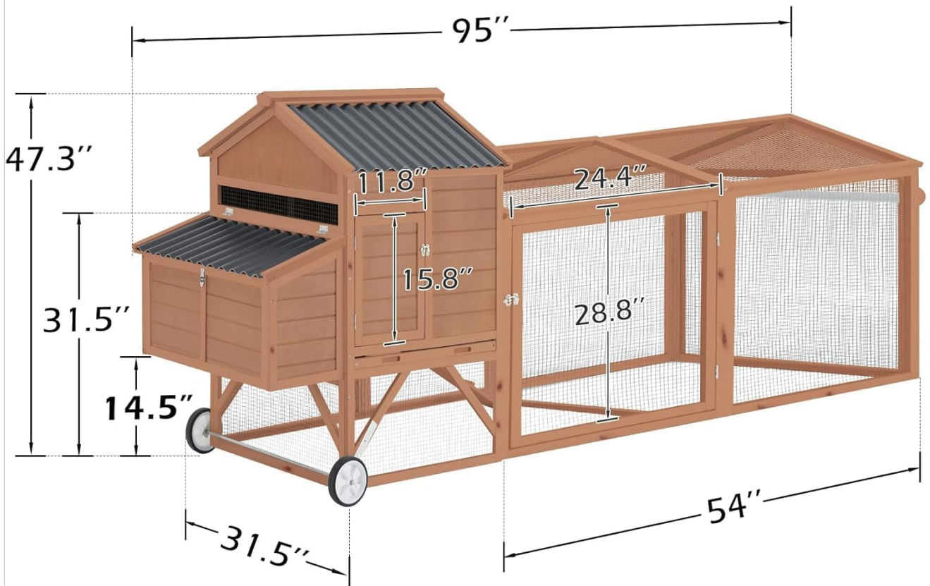
Figure 6.1: Detailed product dimensions of the AECOJOY chicken coop.
