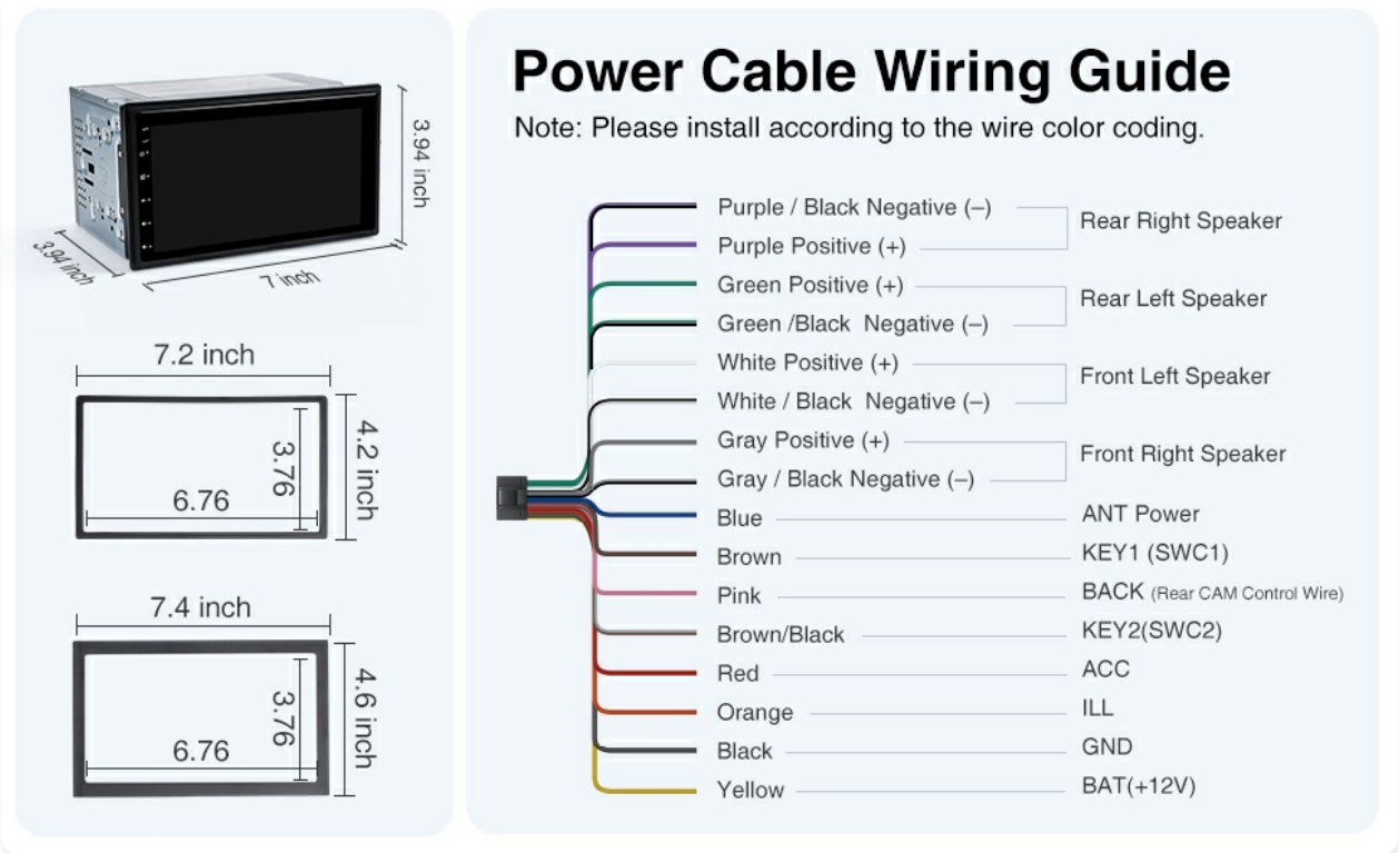
Figure 3: A detailed diagram illustrating the power cable wiring for the AINAVI car stereo, showing connections for speakers, ANT power, SWC, ACC, ILL, GND, and BAT (+12V).
