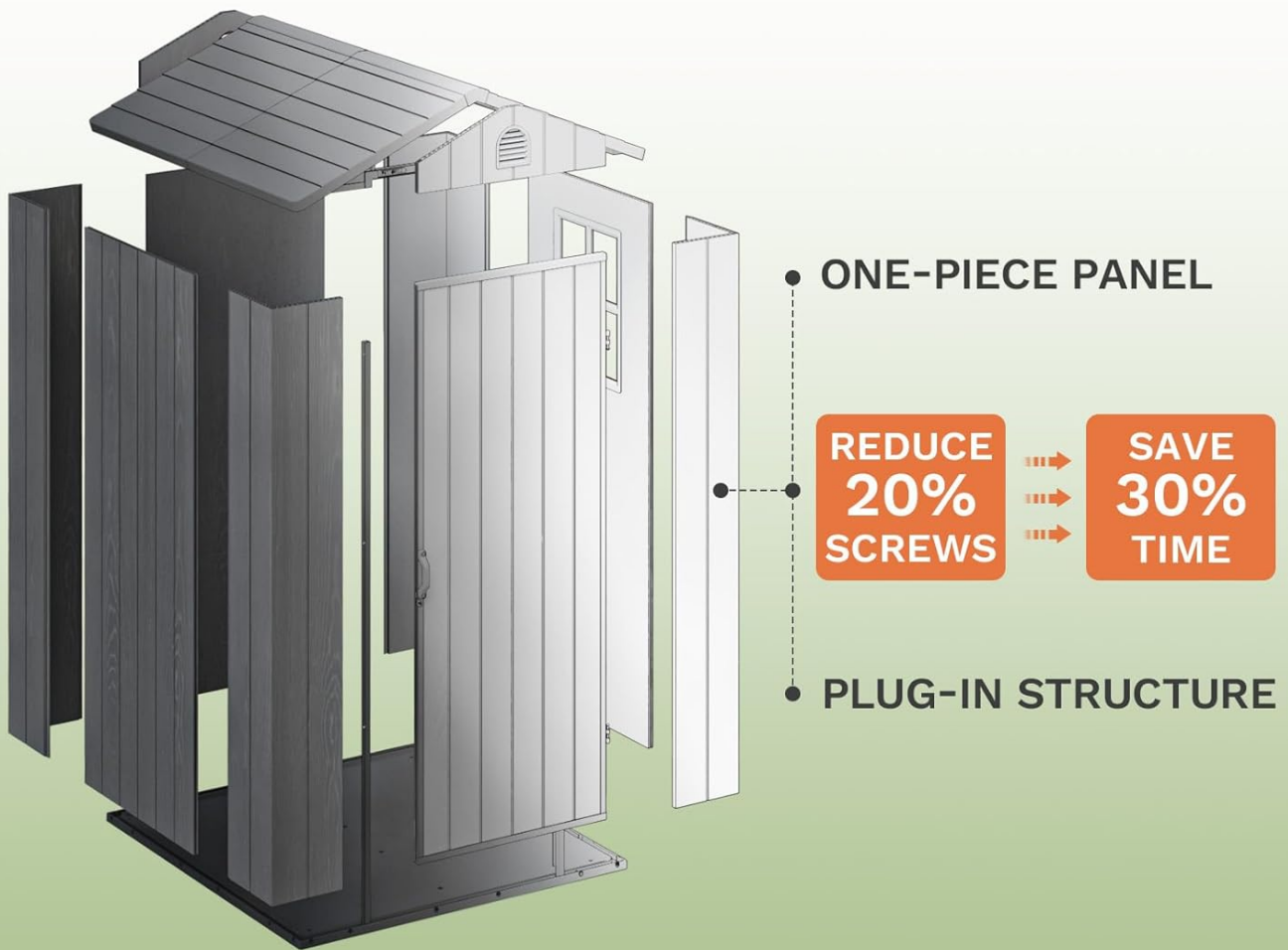
Figure 4.3: Exploded view illustrating the one-piece panel and plug-in construction for easy assembly.
