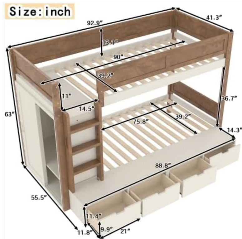
Figure 2.1: Overall dimensions of the bunk bed, including length, width, and height of each section, and drawer measurements.
