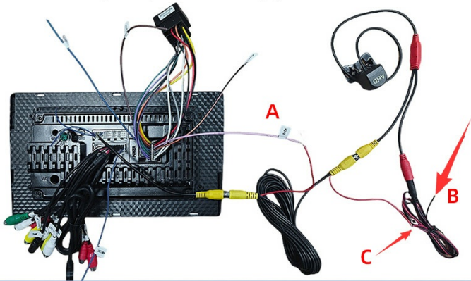
Image: Wiring diagram for the backup camera.
