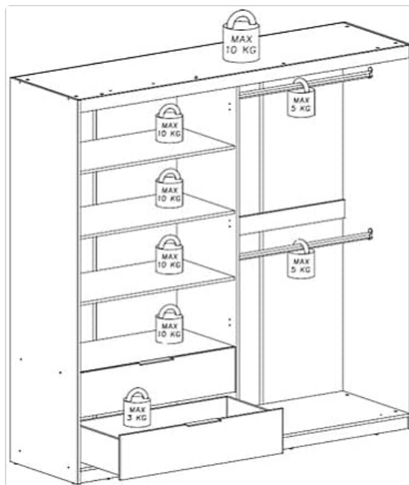
Image 5.1: Load capacity guidelines. Each shelf can hold up to 10 kg, each hanging rail up to 5 kg, and each drawer up to 3 kg.
