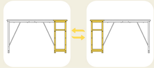
Figure 3: Technical diagram for shelf assembly and placement.
