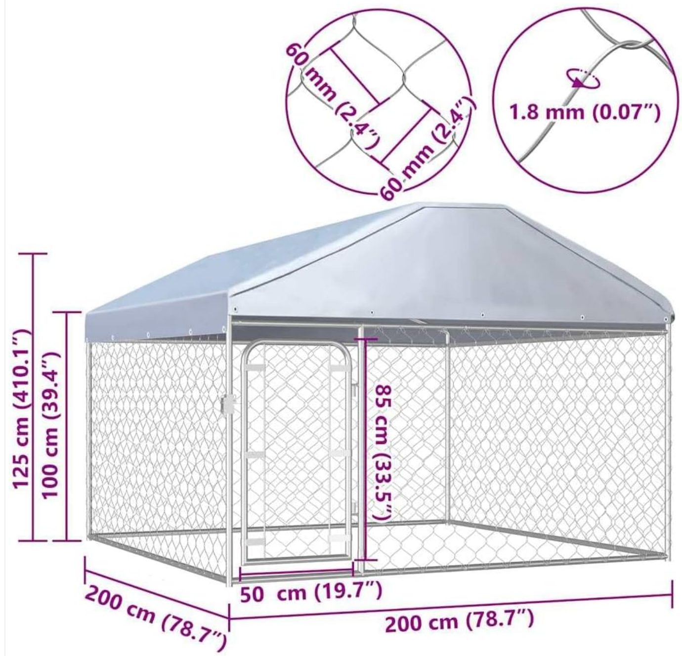
Figure 3: A technical diagram illustrating the overall dimensions of the kennel, including length, width, height, and door opening measurements.
