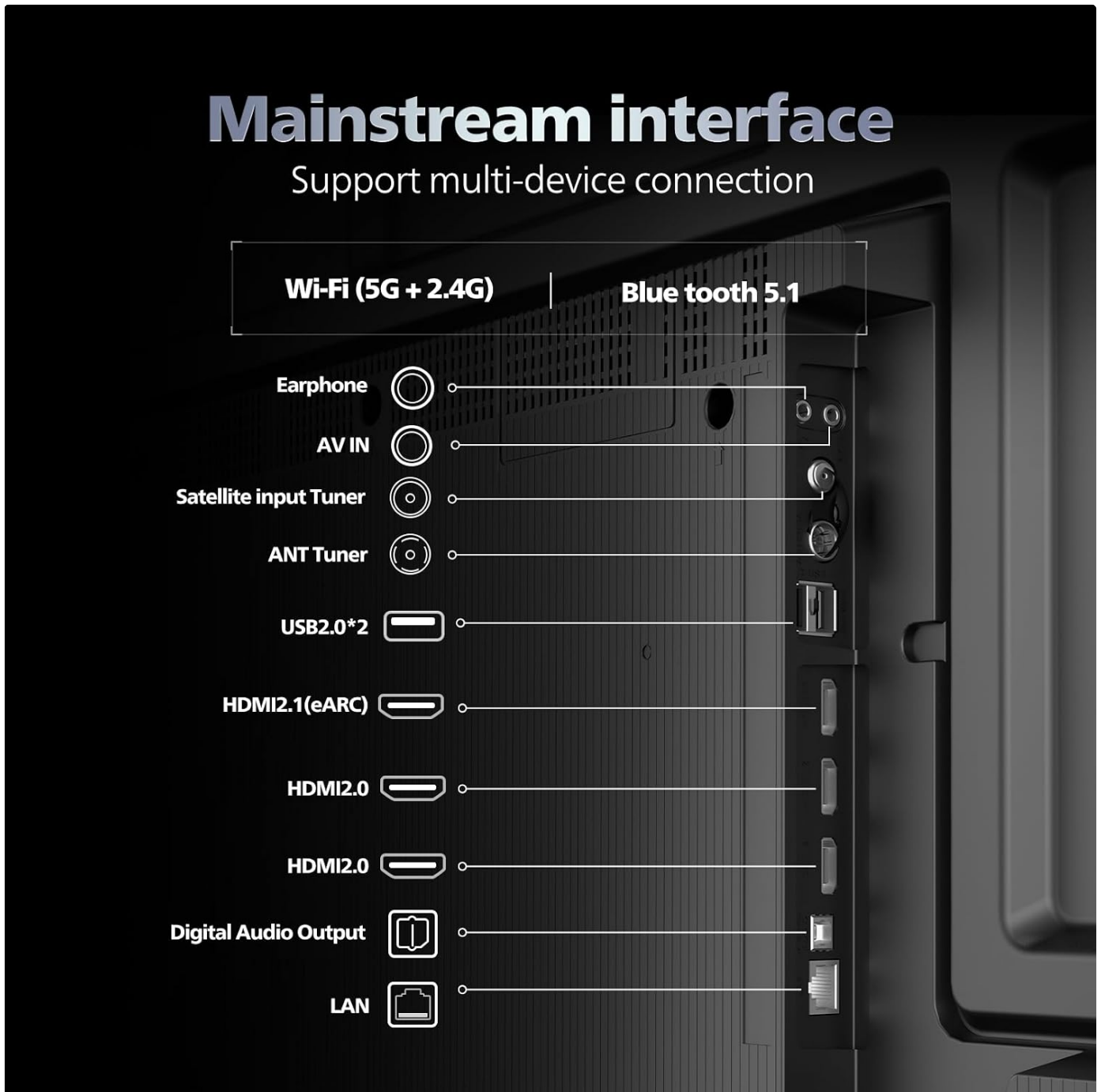
Rear view of the television, highlighting the mounting points and various input/output ports.
