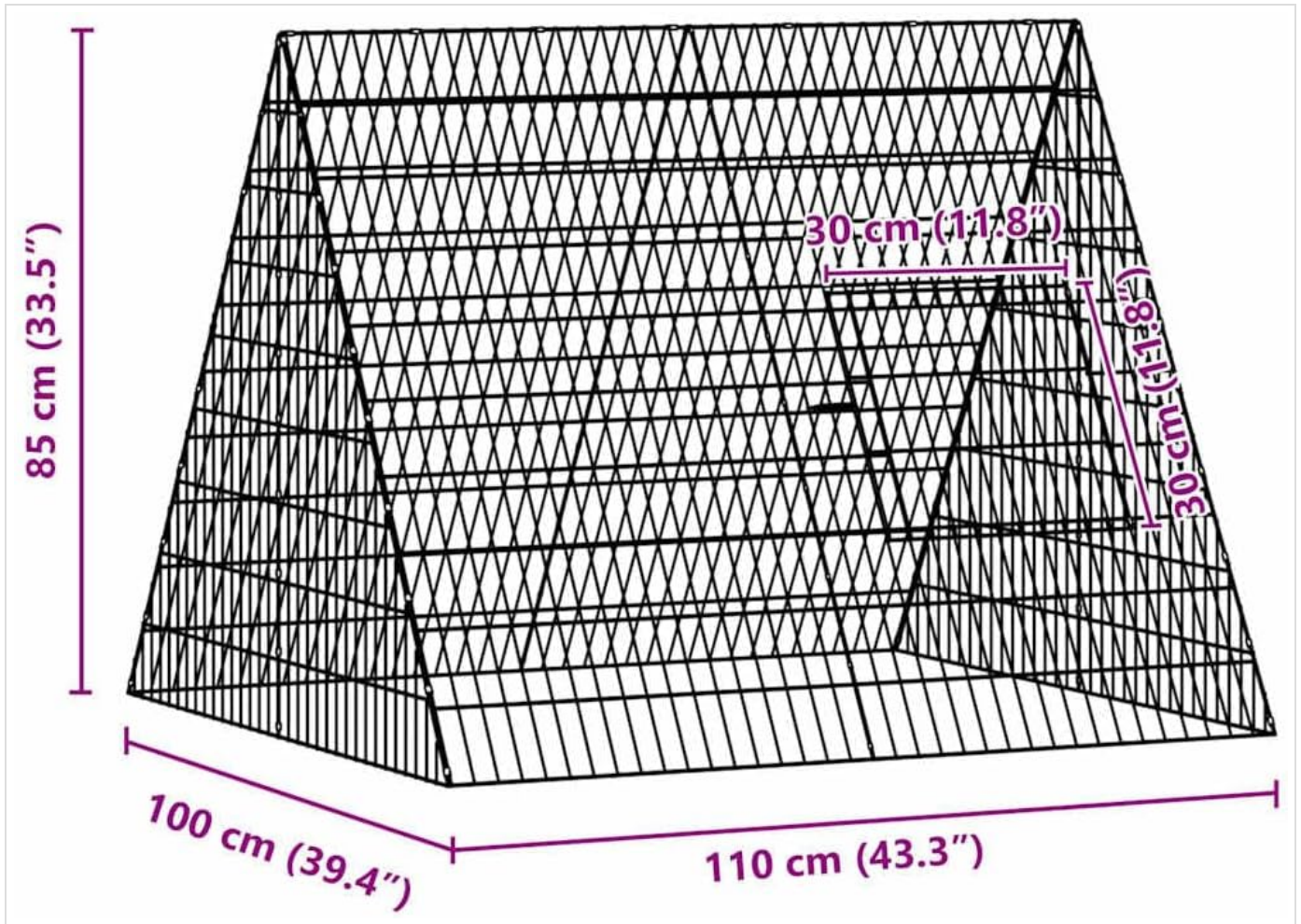
Image: A diagram illustrating the overall dimensions of the chicken cage: 110 cm (43.3") length, 100 cm (39.4") width, and 85 cm (33.5") height. It also shows a 30 cm (11.8") opening.
