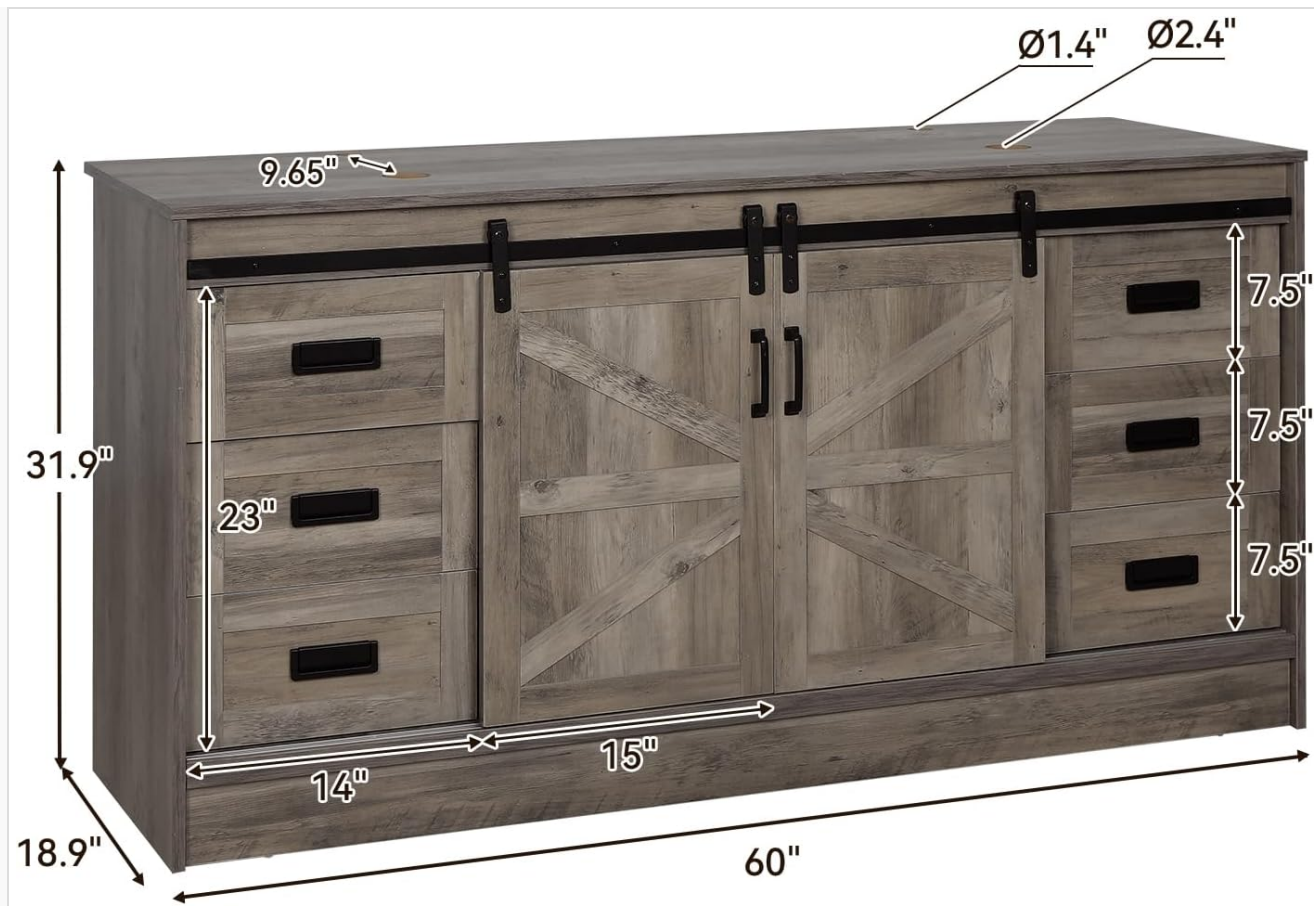
Image 2.2: Detailed dimensions of the vanity cabinet and sink placement.
