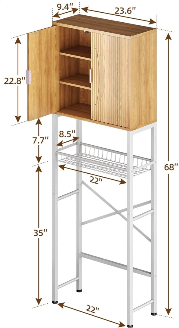
Figure 2: Detailed product dimensions for planning placement.
