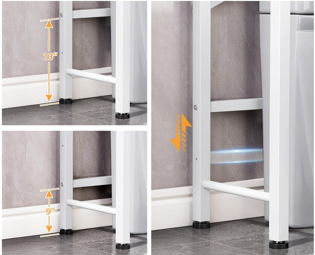
Figure 3: The adjustable bottom bar can be moved up or down to clear water pipe valves.
