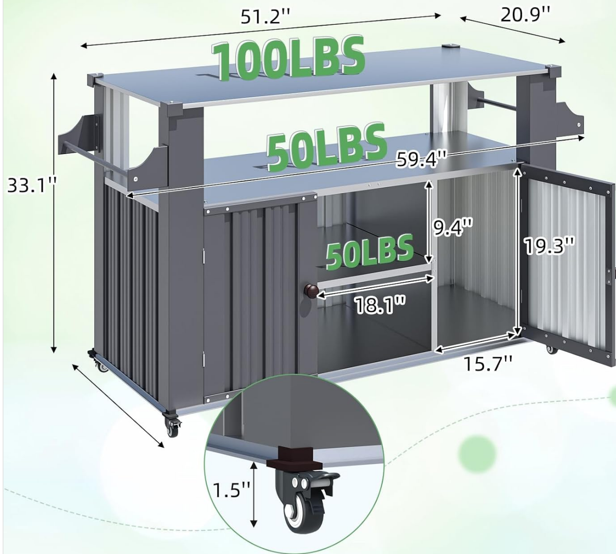
Image: A detailed diagram illustrating the overall product dimensions and internal storage measurements.
