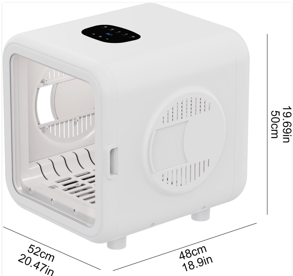
Figure 4: Dimensions of the advwin 75L Automatic Pet Dryer Box, showing approximate measurements in inches and centimeters.
