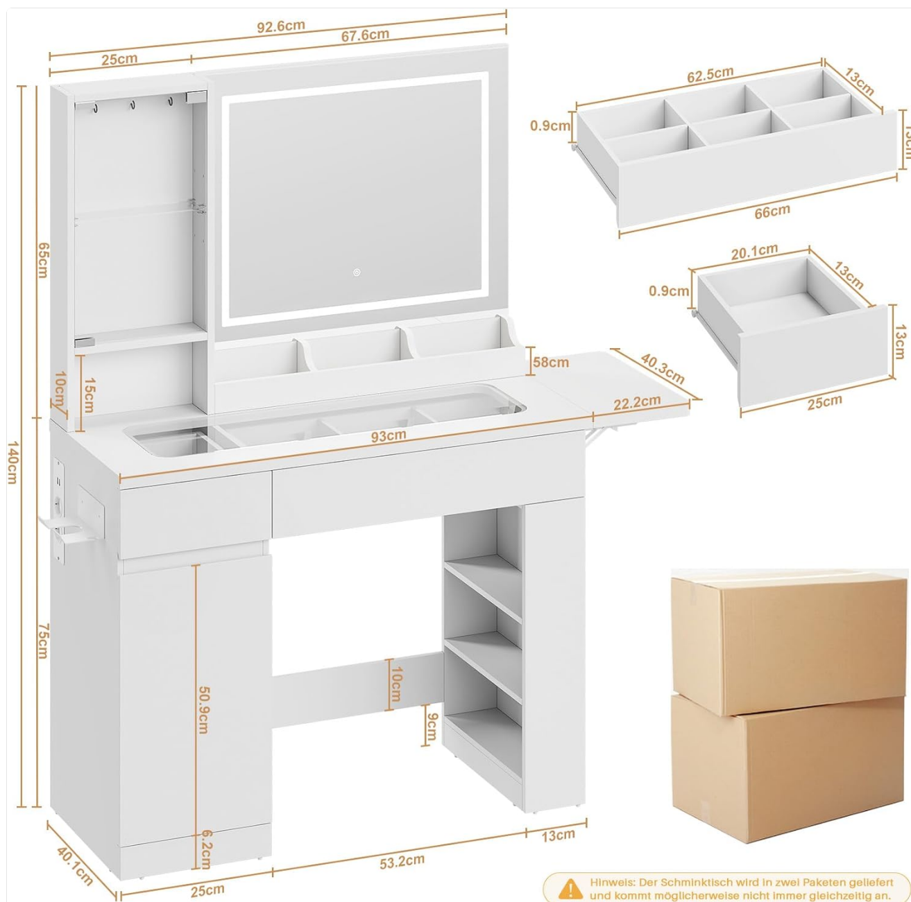
Figure 1: Overview of dressing table dimensions and typical packaging. The product is delivered in two separate packages.
